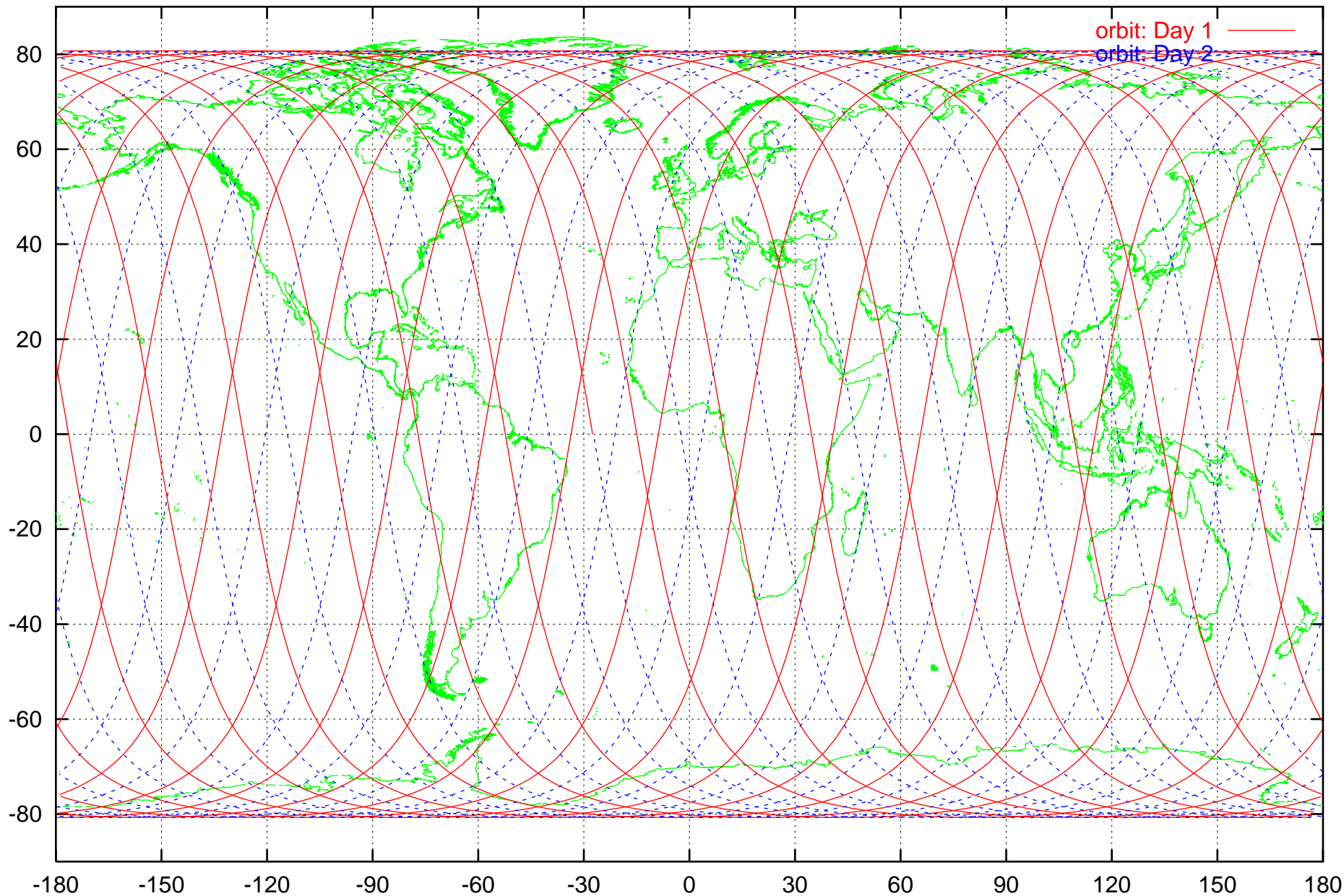
Ground Trace of ROCSAT-2 at the Packing Orbit : 723 Km, 29 loops / 2 days
